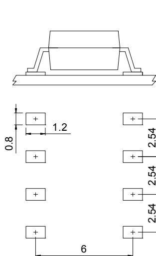
8-pin SOP
