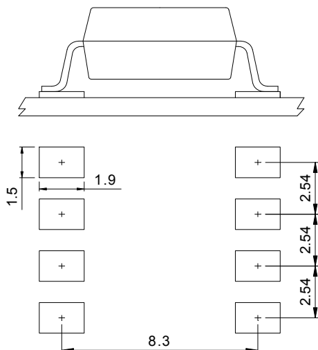
8-pin SMD
